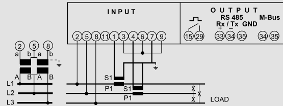
Three-phase 3Ph network, unbalanced load (aron L1-L2)
