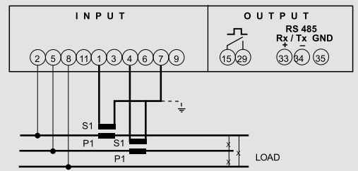
Three-phase 3Ph network, unbalanced load (aron L1-L2)
