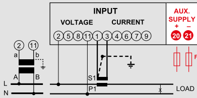
Single phase network
