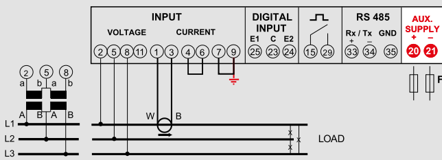
3-phase network, 3 wire, 1 System
