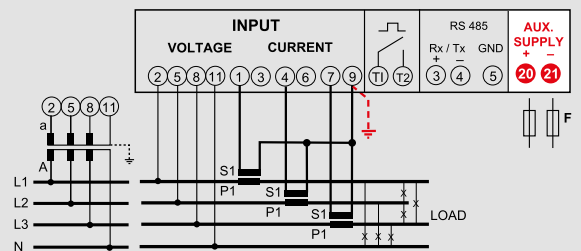
3-phase network, 4 wire
